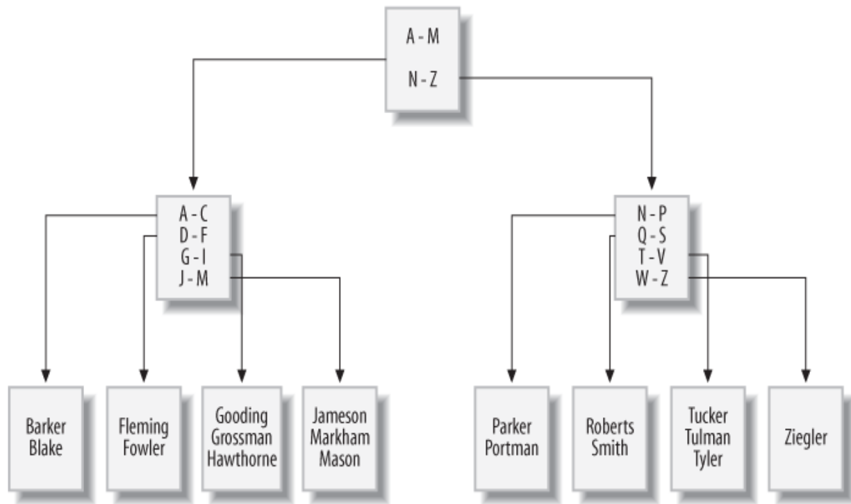
Figure 13-1. B-tree example
